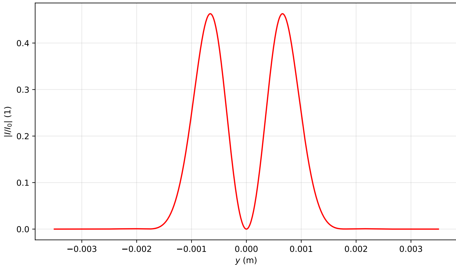
Intensity profile I(x=0, y, z=1.831)/I_0 , P_{in}=2.0P_{cr} , artificial time
